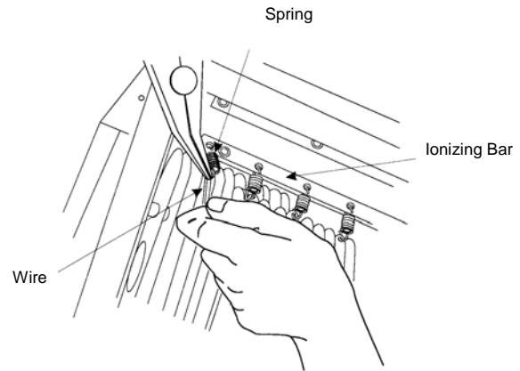
Fig. 6 — Replacing An Ionizing Wire
