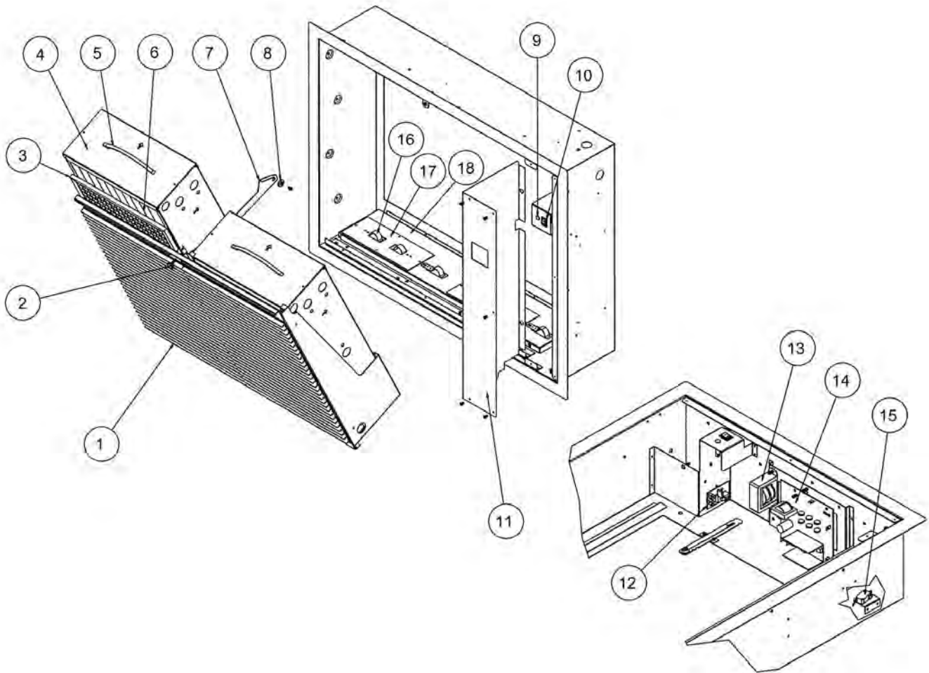
Fig. 8 — Exploded View and Parts List
