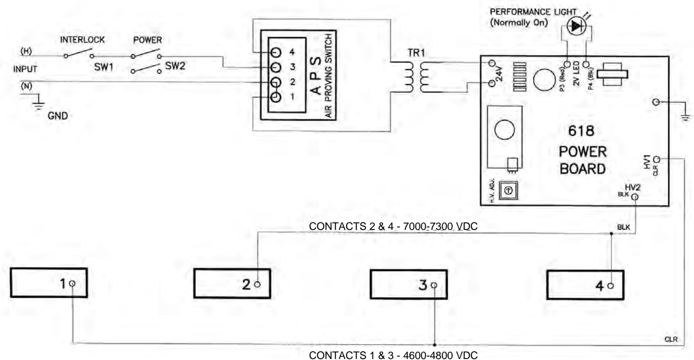
Fig. 5 — Schematic
